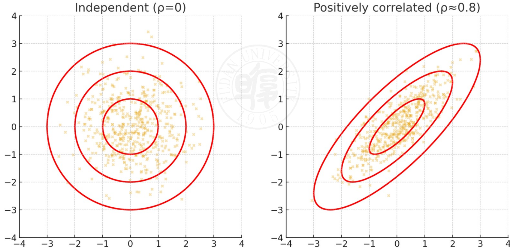
2D Gaussian: effect of covariance / correlation
